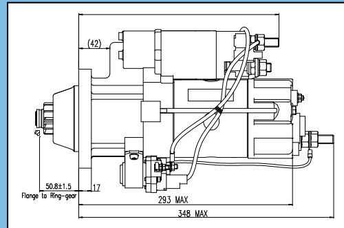
Side Dimensional
