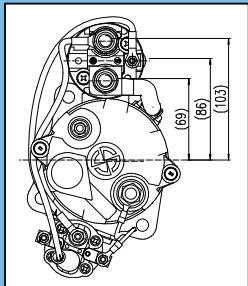
Rear Dimensional
