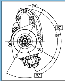
Front Dimensional
